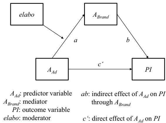
conditional indirect effect: indirect effect ab , conditional on levels of elabo being high (1) or low (2) Fig. 16: Moderated mediation example (PROCESS model 7)
